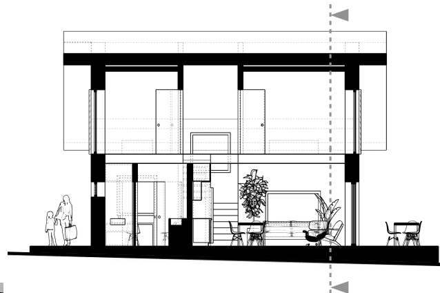
west section
