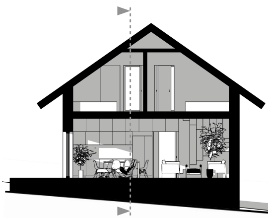
south section
